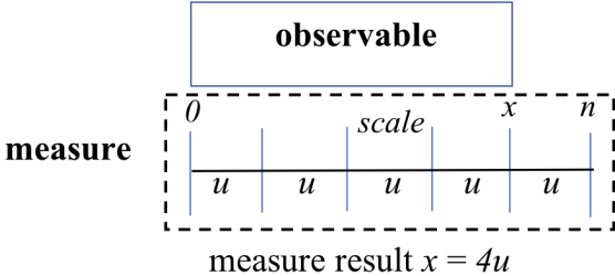
Figure 2. Representational theory
